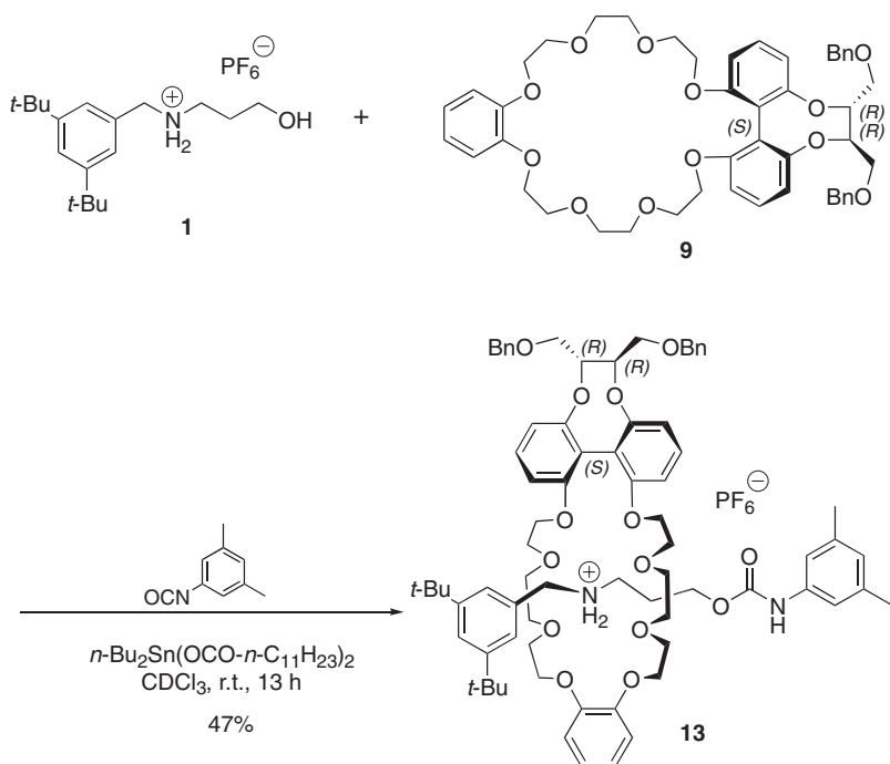
Scheme 6. Synthesis of optically-active [2]rotaxane ( 13 ).
