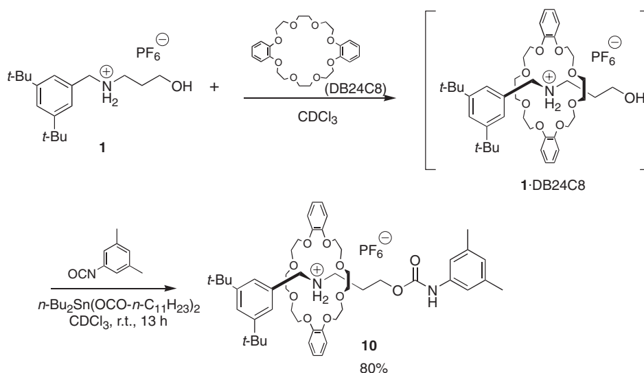
Scheme 4. Synthesis of [2]rotaxane ( 10 ).
