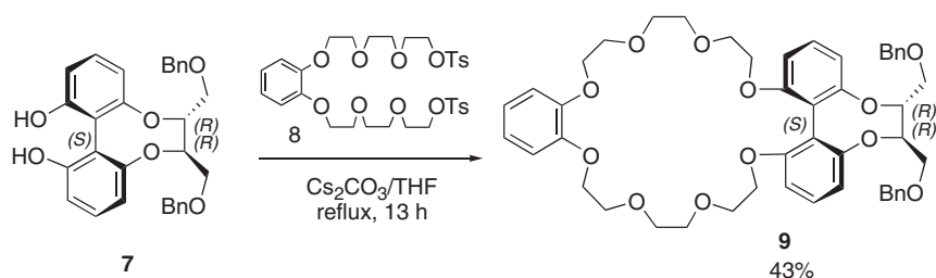
Scheme 3. Synthesis of optically-active 26-membered crown ether ( 9 ).
