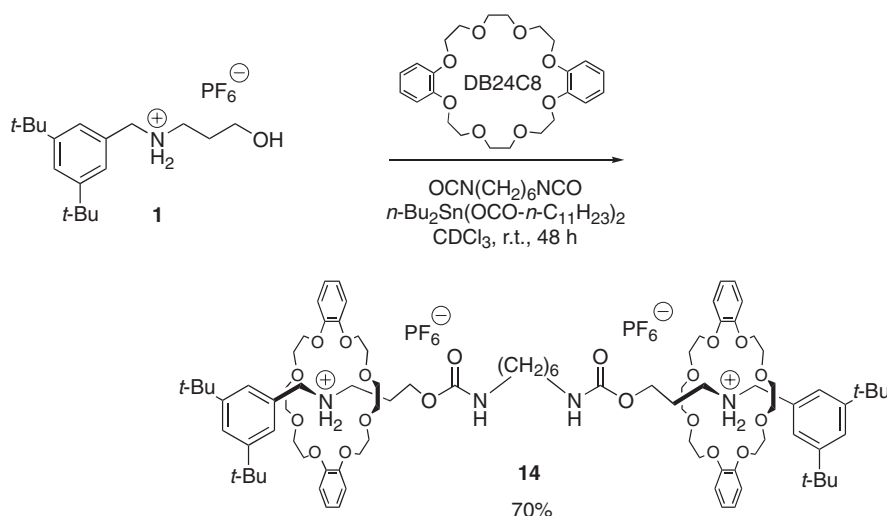
Scheme 7. Synthesis of [3]rotaxane ( 14 ).
