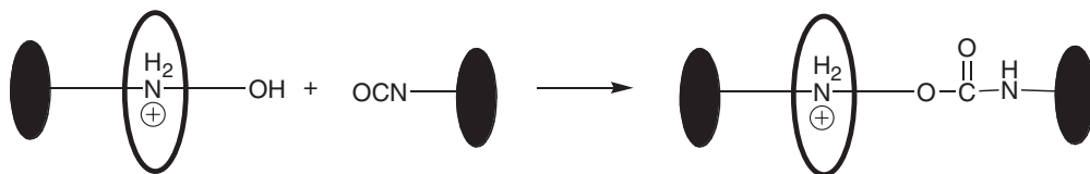
Scheme 1. A schematic representation of the synthetic protocol for [2]rotaxanes utilizing urethane formation from alcohol and isocyanate based on sec -ammonium/crown motif.
