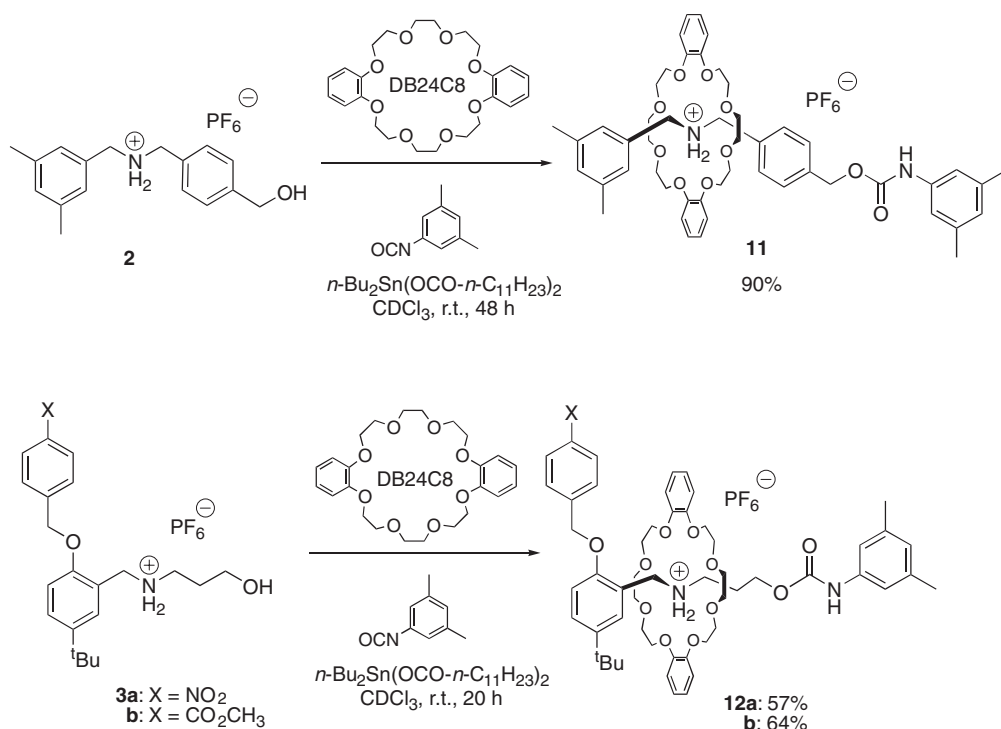
Scheme 5. Synthesis of [2]rotaxane ( 11 and 12 ).
