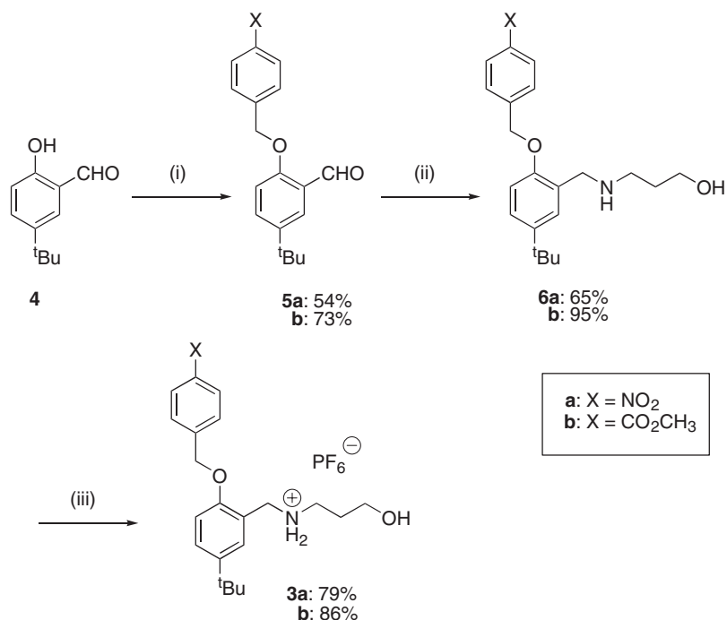
Scheme 2. Reagents and conditions: (i) 4-nitrobenzyl chloride for 5a , methyl 4-bromomethylbenzoate for 5b , NaH/DMF, 100 °C; (ii) 3-amino-1-propanol/toluene, then NaBH 4 /MeOH; (iii) 5% HPF 6 aq, 0 °C.
